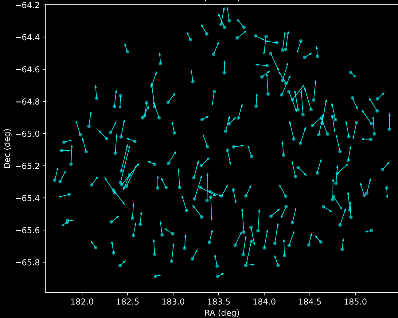
GALAH DR4 Noise Stream Proper Motion Vectors (n=167)
