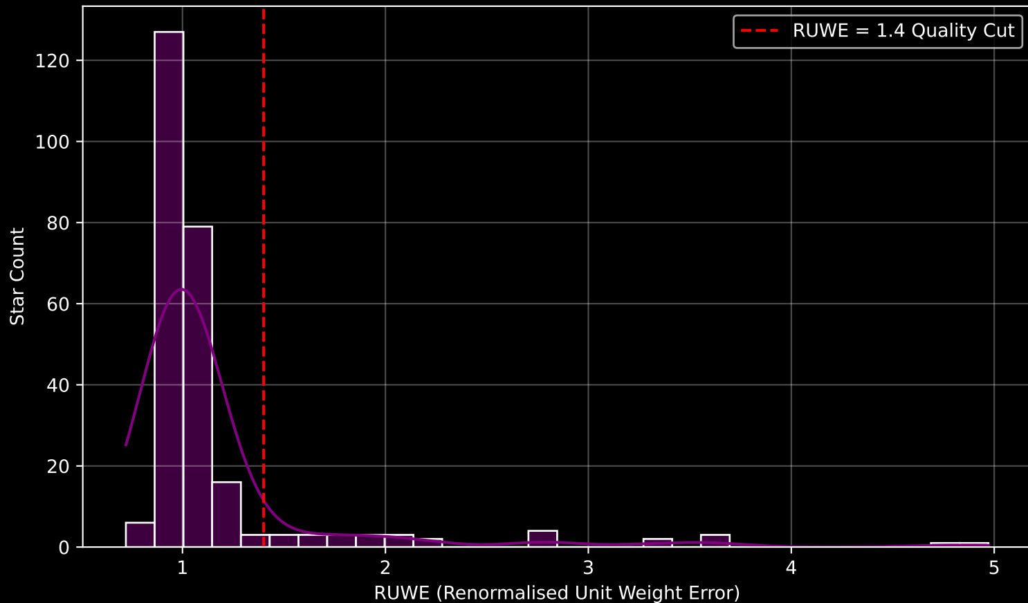
GALAH DR4 Field [681] RUWE Distribution (n= 259)
