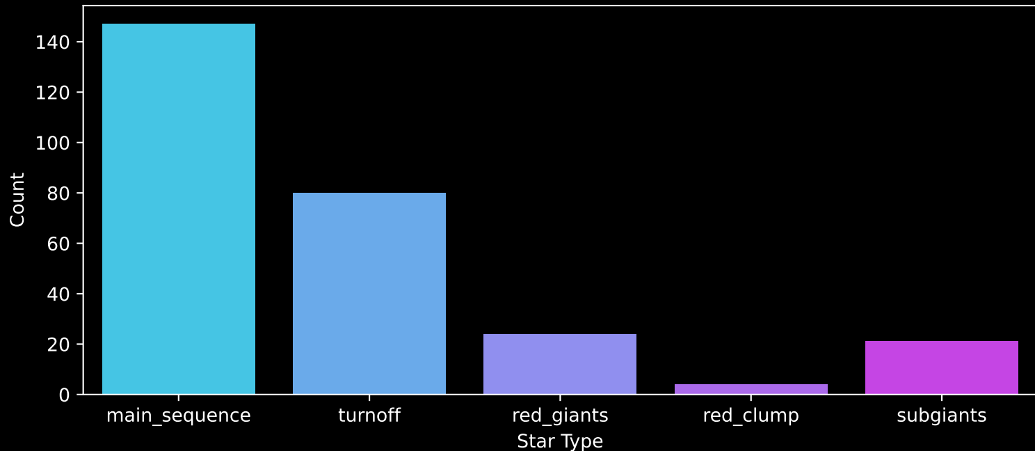
GALAH DR4 Field: [681] Count plot of Star Type
