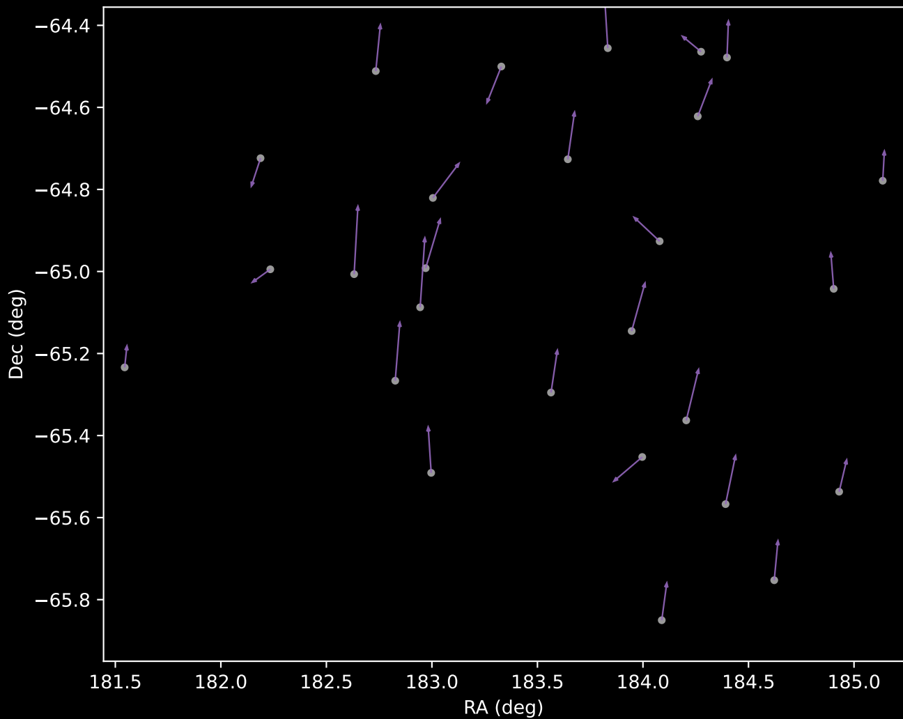
GALAH DR4 Cluster 8 Proper Motion Vectors (n=27)
