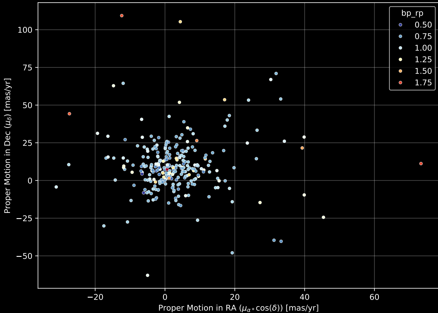
GALAH DR4 Field: [681] Proper Motion Diagram (n= 276)
